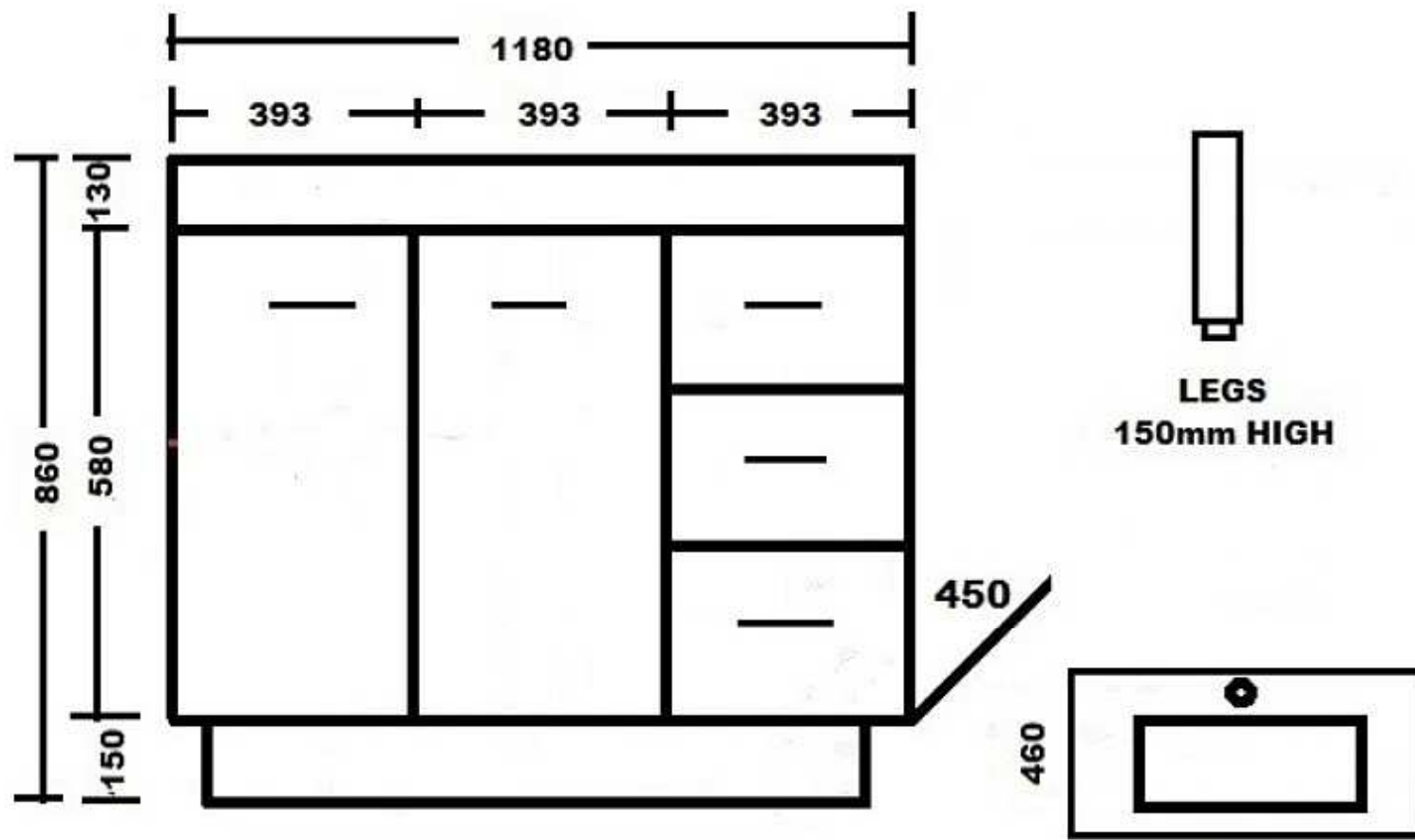
1200 ORION / LINDA CABINET
