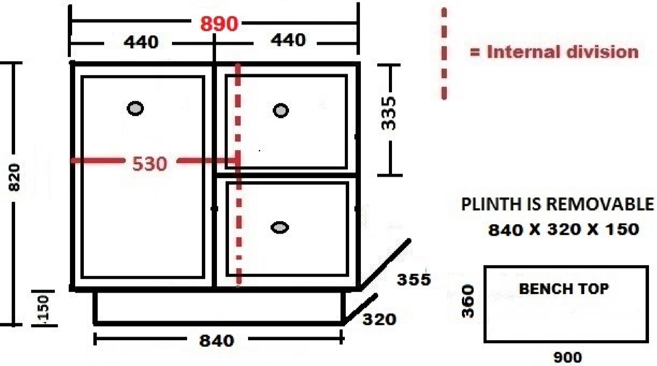
900 STAMFORD CABINET
